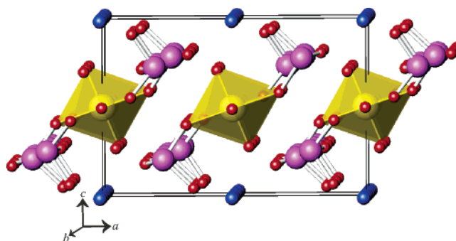
Figure 5. Packing diagram for \text{Na}_2[\text{UO}_2(\text{IO}_3)_4(\text{H}_2\text{O})] .
