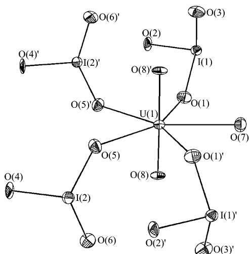
Figure 1. View of the structure of the [\text{UO}_2(\text{IO}_3)_4(\text{H}_2\text{O})]^{2-} anion in \text{Na}_2[\text{UO}_2(\text{IO}_3)_4(\text{H}_2\text{O})] , which has imposed 2-fold symmetry. 50% probability ellipsoids are depicted.
