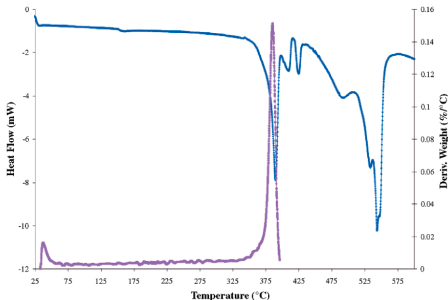
Figure 6. DSC and TGA thermograms of \text{Na}_2[\text{UO}_2(\text{IO}_3)_4(\text{H}_2\text{O})] .
