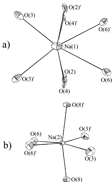
Figure 4. (a) View of the distorted dodecahedral environment around Na(1) and (b) the distorted octahedral environment around Na(2) in \text{Na}_2[\text{UO}_2(\text{IO}_3)_4(\text{H}_2\text{O})] . The environments around the \text{Na}^+ cations are consistent with a polar structure.
