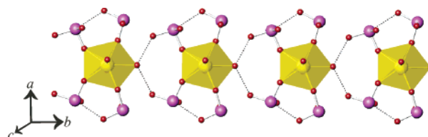
Figure 3. Depiction of the one-dimensional chains of [\text{UO}_2(\text{IO}_3)_4(\text{H}_2\text{O})]^{2-} anions formed through intermolecular hydrogen bonds between the coordinating water molecule and oxo atoms of iodate from adjacent anions. The dashed lines between iodate anions within individual [\text{UO}_2(\text{IO}_3)_4(\text{H}_2\text{O})]^{2-} anions indicate iodate...iodate interactions that orient the iodate anions along the b axis. Therefore, cooperative interactions are present for aligning different groups the structure of \text{Na}_2[\text{UO}_2(\text{IO}_3)_4(\text{H}_2\text{O})] , where the hydrogen bonding, intermolecular iodate...iodate interactions, and the lone-pair alignment contribute to the short-range and long-range polarity.
