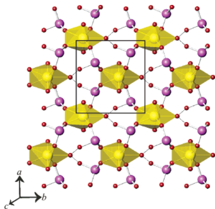
Figure 2. Illustration of [\text{UO}_2(\text{IO}_3)_4(\text{H}_2\text{O})] units found in \text{UO}_2(\text{IO}_3)_2(\text{H}_2\text{O}) .
